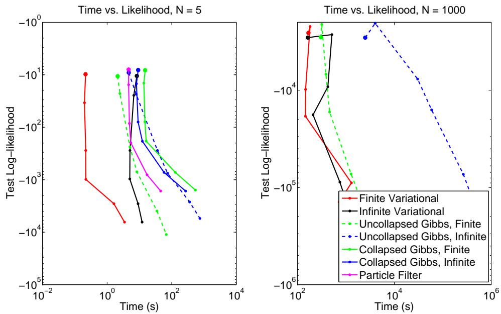
Figure 6: Time versus log-likelihood plot for K = 20 . The larger dots correspond to D = 5 the smaller dots to D = 10, 50, 100, 500, 1000 .
