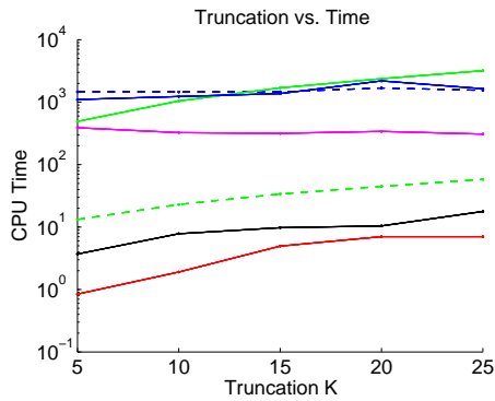
Figure 5: Time versus truncation ( K ). The variational approaches are generally orders of magnitude faster than the samplers (note log scale on the time axis).
