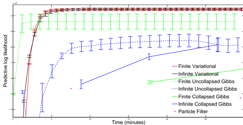
Figure 3: Evolution of test log-likelihoods over a thirty-minute interval for N = 500 , D = 500 , and K = 20 . The finite uncollapsed Gibbs sampler has the fastest rise but gets caught in a lower optima than the variational approach.
