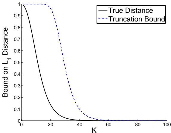
Figure 2: Truncation bound and true L_1 distance.
