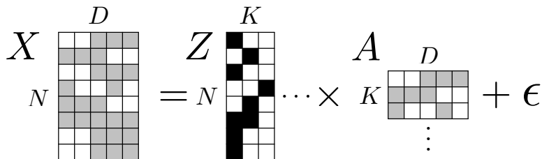
Figure 1: Our likelihood model posits that the data \mathbf{X} is the product \mathbf{Z}\mathbf{A} plus some noise.
