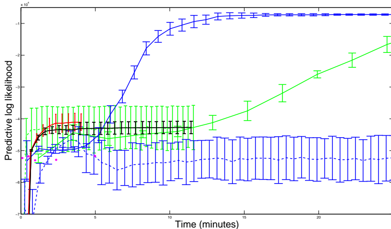
Figure 4: Evolution of test log-likelihoods over a thirty-minute interval for N = 100 , D = 500 , and K = 25 . For smaller N , the Gibbs sampler does better at finding an optima of high probability mass.
