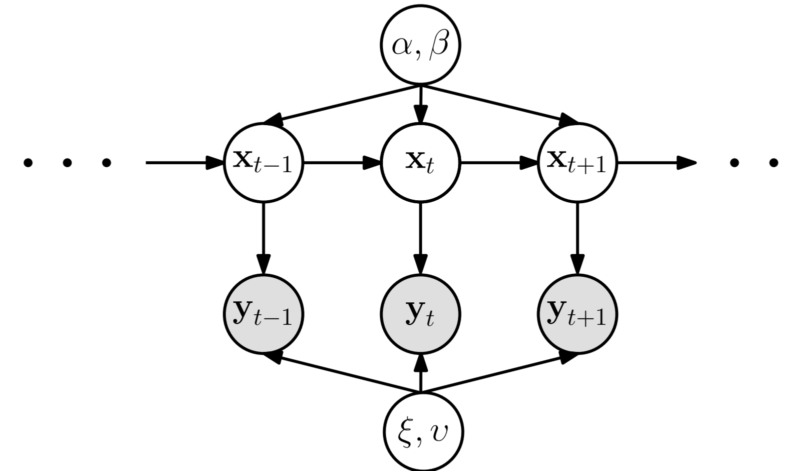
FIGURE 2: The free parameters \alpha, \beta and \xi, \nu serve as a pseudo training set for \mathcal{GP}_f and \mathcal{GP}_g , respectively. \mathcal{GP}_f and \mathcal{GP}_g are not full GPs, but rather sparse GPs that impose the condition \mathbf{x}_{t+1} \perp \mathbf{x}_{t-1} | \mathbf{x}_t, \alpha, \beta during predictions.
