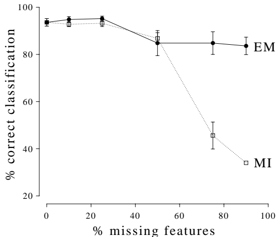
Classification with missing inputs
