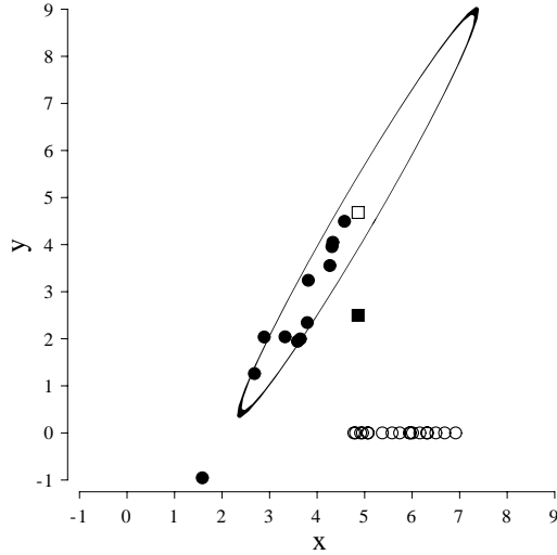
Figure 1: A simple example. Complete data were generated from a Gaussian with mean (5, 5) and covariance matrix \begin{pmatrix} 5/4 & 9/4 \\ 9/4 & 17/4 \end{pmatrix} . Data points with missing y values are denoted by hollow circles on the y = 0 line. The solid square indicates the (x, y) mean calculated over the observed data. The hollow square and the ellipse indicate the mean and standard deviation calculated from the incomplete data using a maximum likelihood (ML) algorithm. Note that the ML estimate of \mu_y is higher than any of the observed values of y !
