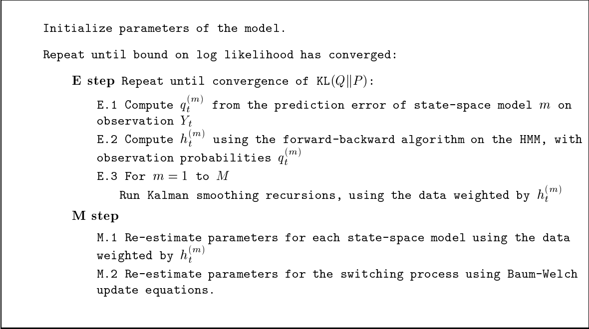
Figure 5: Learning algorithm for switching state-space models.
