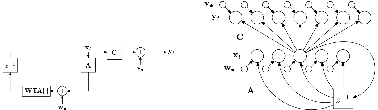
Figure 3: Discrete state generative model for dynamic data. The \mathbf{WTA}[\cdot] block implements the winner-take-all nonlinearity. The z^{-1} block is a unit delay. The covariance matrix of the input noise \mathbf{w} is \mathbf{Q} and the covariance matrix of the output noise \mathbf{v} is \mathbf{R} . In the network model below, the smaller circles represent noise sources and the hidden units \mathbf{x} have a winner take all behaviour (indicated by dashed lines). Outgoing weights have only been drawn from one hidden unit. This model is equivalent to a hidden Markov model with tied output covariances.
