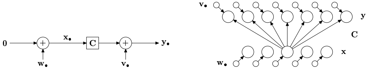
Figure 2: Static generative model (continuous state). The covariance matrix of the input noise \mathbf{w} is \mathbf{Q} and the covariance matrix of the output noise \mathbf{v} is \mathbf{R} . In the network model below, the smaller circles represent noise sources and all units are linear. Outgoing weights have only been drawn from one hidden unit. This model is equivalent to factor analysis, SPCA and PCA models depending on the output noise covariance. For factor analysis, \mathbf{Q} = \mathbf{I} and \mathbf{R} is diagonal. For SPCA, \mathbf{Q} = \mathbf{I} and \mathbf{R} = \alpha \mathbf{I} . For PCA, \mathbf{Q} = \mathbf{I} and \mathbf{R} = \lim_{\epsilon \rightarrow 0} \epsilon \mathbf{I} .
