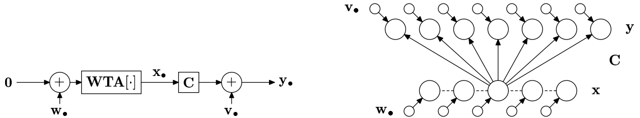
Figure 4: Static generative model (discrete state). The WTA[.] block implements the winner-take-all nonlinearity. The covariance matrix of the input noise \mathbf{w} is \mathbf{Q} and the covariance matrix of the output noise \mathbf{v} is \mathbf{R} . In the network model below, the smaller circles represent noise sources and the hidden units \mathbf{x} have a winner take all behaviour (indicated by dashed lines). Outgoing weights have only been drawn from one hidden unit. This model is equivalent to a mixture of Gaussian clusters with tied covariances \mathbf{R} or to vector quantization (VQ) when \mathbf{R} = \lim_{\epsilon \rightarrow 0} \epsilon \mathbf{I} .
